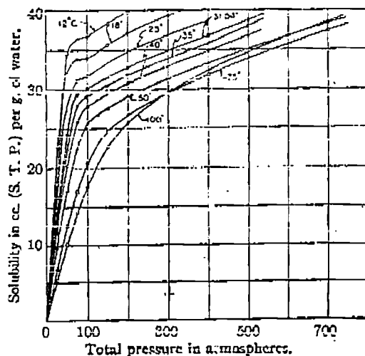
Fig. 4.—Solubility of carbon dioxide in water.
