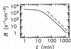
FIG. 4. Rate of rearrangement events vs foam age. The dashed line has slope -2 and shows that R exhibits scaling behavior.
