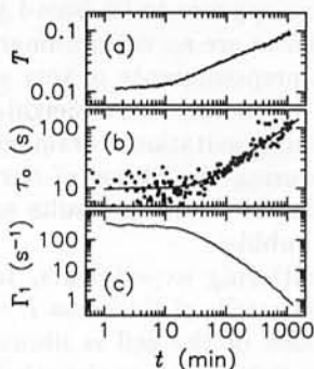
FIG. 2. Typical multiple light-scattering data vs foam age: (a) the average static transmission T through a sample of thickness L = 0.7 \text{ cm} , (b) \tau_0 from dynamic backscattering from a sample of thickness L = 1.0 \text{ cm} , and (c) \Gamma_1 from dynamic transmission with L = 0.4 \text{ cm} . All three data sets exhibit nearly power-law behavior after about 20 min.
