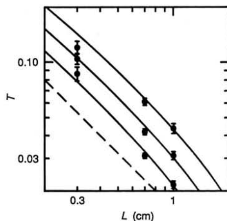
Fig. 2. Transmission versus foam thickness at 40, 90, and 200 min of age for wavelength \lambda = 488.0 \text{ nm} ; error bars are \pm 1 standard deviation based on 10 to 50 measurements. With increasing age, more light is transmitted. The dashed line shows the form of T \propto 1/L . The solid curves are the best fits to Eq. 1.
